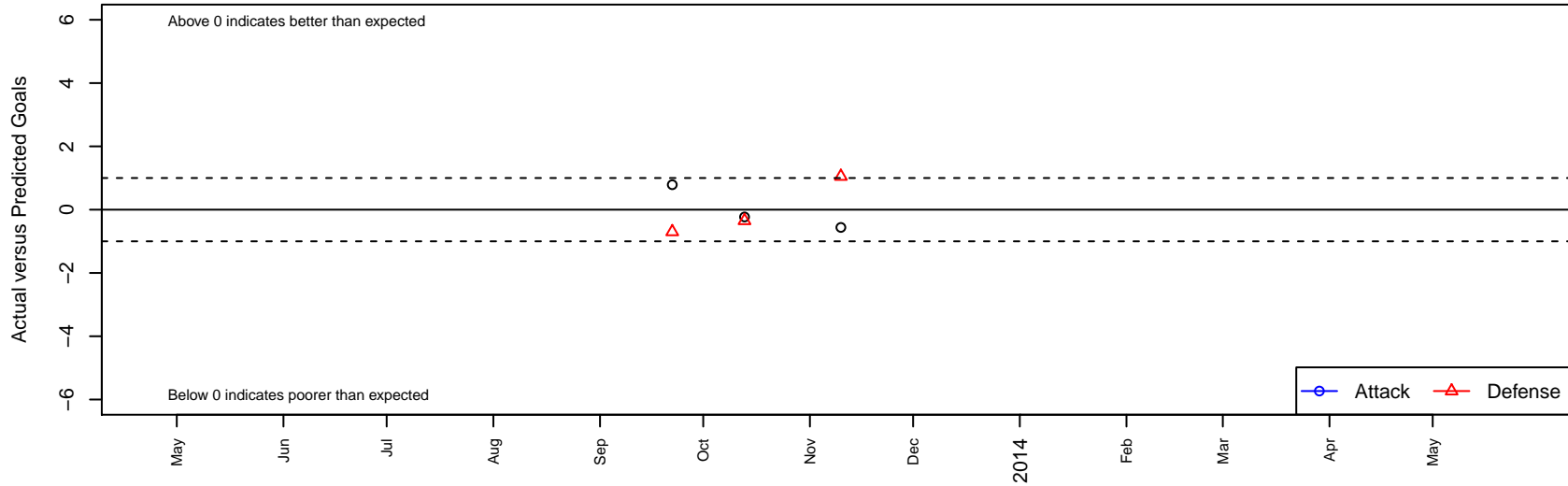
Tracy Blaze G99 Dots are actual minus expected GF (blue circles) and GA (red triangles). Blue line is smoothed change in attack strength. Red is smoothed change in defense strength.
